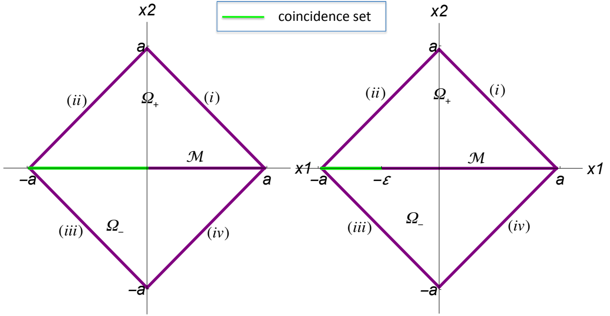
Figure 3: Domains \Omega_+ and \Omega_- ; coincidence sets for u and v_1 (left) and for v_{3,\epsilon} (right)
