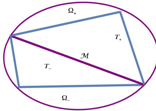
Figure 2: Triangles T_+ and T_-
