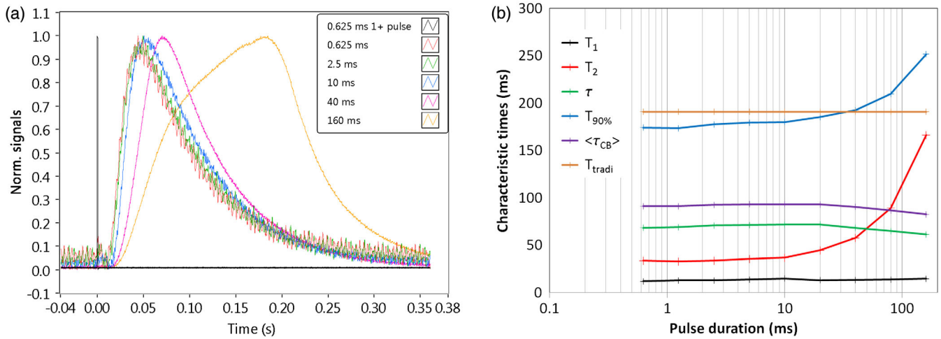
FIG. 5. (a) 0.625 ms pulse command and normalized Rb 19+ response to 0.625, 2.5, 10, 40, and 160 ms 1+ pulses. (b) Characteristic times as a function of the 1+ pulse duration. Characteristic time parameters uncertainty is evaluated at \pm 3\% .
