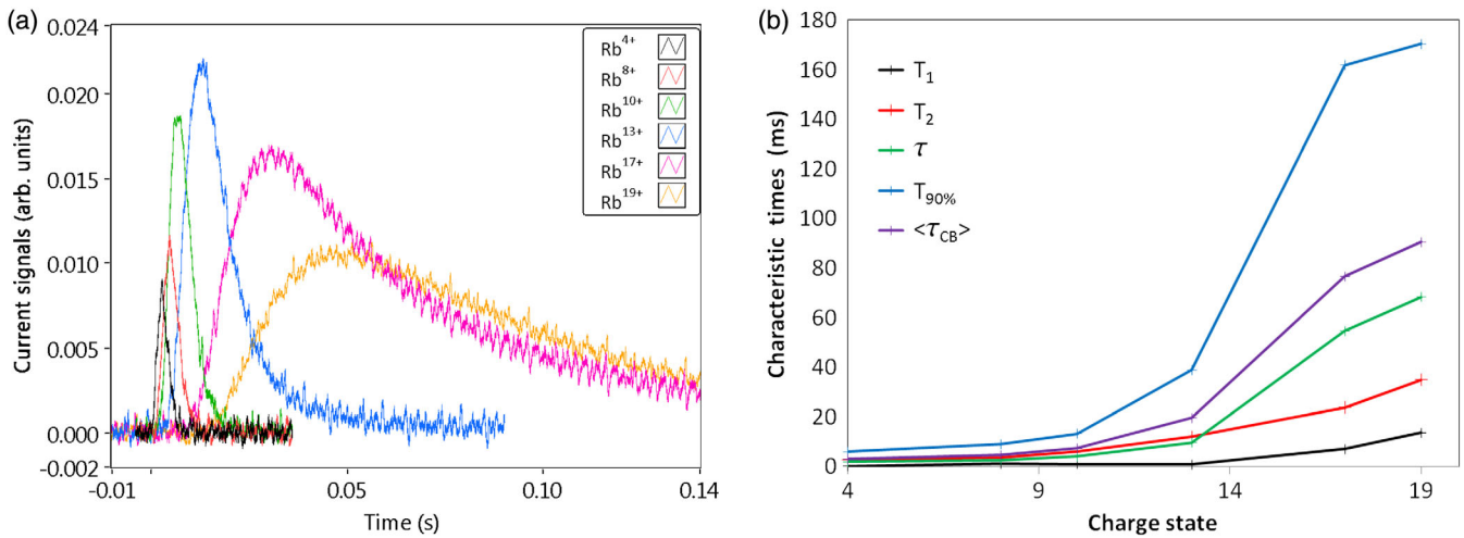
FIG. 6. (a) Rb 4+ , Rb 8+ , Rb 10+ , Rb 13+ , Rb 17+ , and Rb 19+ beam intensities responses to a 2.5 ms pulse. (b) Evolution of the characteristic times as a function of the Rb charge state. The characteristic time parameters uncertainty is evaluated at \pm 3\% .
