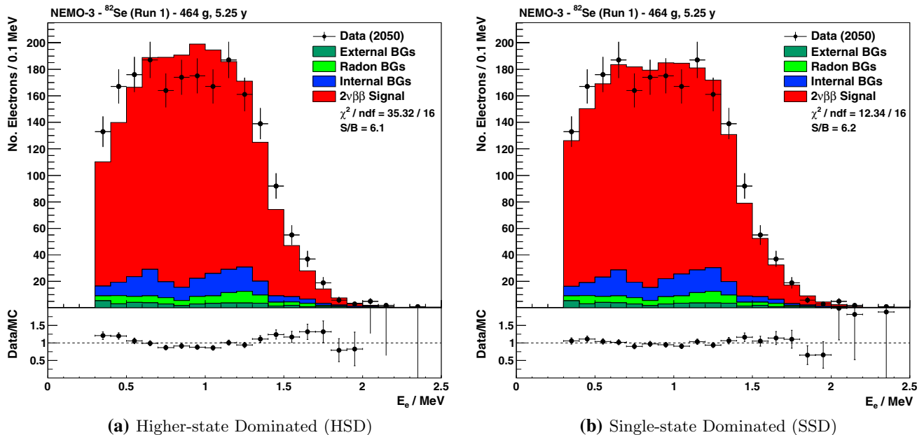
Fig. 7 Energy distribution of individual electrons in the \beta\beta channel for foils from enrichment run 1, after removing events where \Sigma E_e < 1.6\text{ MeV} to reduce the effect of contamination by ^{234m}\text{Pa} . The data are compared to the predicted spectrum from MC under the
