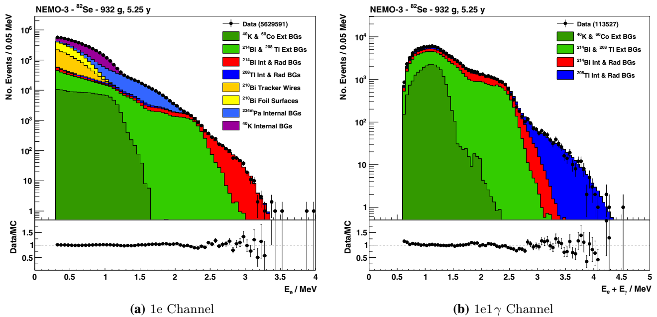
Fig. 4 a Energy spectrum of electrons in events containing a single electron selected in the 1e channel compared to the MC prediction. At energies below 1 MeV the dominant contributions are from ^{40}\text{K} contamination and from ^{210}\text{Bi} deposited on the surfaces of the source foils and tracker wires. The contribution from ^{234\text{m}}\text{Pa} becomes significant in an intermediate region at 1.2–2.2 MeV. Above this energy the spectrum is composed of events from ^{214}\text{Bi} originating from source foil contamination and radon backgrounds. The small numbers of events at
