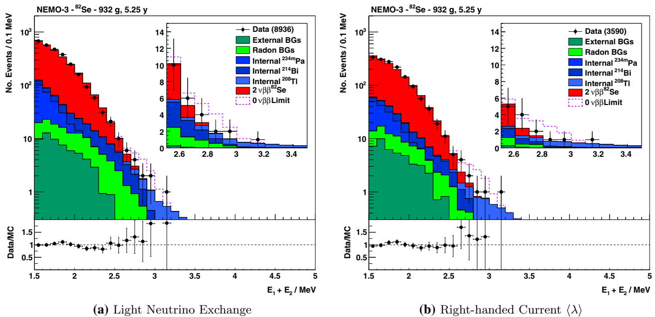
Fig. 10 Distribution of the summed electron energies in the \beta\beta channel and the ratio between the observed and MC predicted data. The inset plot shows the highest energy events on a linear scale. The solid histograms represent the backgrounds and 2\nu\beta\beta predictions and the open histogram shows a hypothetical 0\nu\beta\beta signal corresponding to the limit
