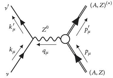
FIGURE 1: A diagram of the neutral-current scattering process. The four momenta of the involved particles are labeled in the figure.
