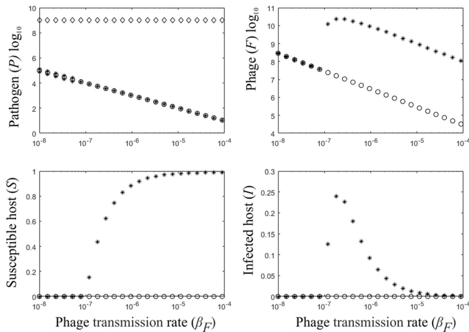
Fig. 1 Bifurcation diagrams of the model dynamics in the absence of the phage-resistant bacteria population ( B = 0 ), presenting equilibrium values of the susceptible host ( S ), the infected hosts ( I ), the pathogen ( P ) and the bacteriophage ( F ) population densities for the phage transmission rate, 10^{-8} < \beta_F < 10^{-4} . The x-axis is log10 scale. When the phage transmission rate is low ( \beta_F < 10^{-7} ), the susceptible and the infected hosts go asymptotically extinct while there is a stable coexistence of the pathogen and the phage. When the phage transmission rate increases, the pathogen population size decreases while the susceptible host population increases, close to their carrying capacity at higher phage transmission rates. The number of the infected hosts abruptly increases as phage transmission increases, but decrease asymptotically towards zero at higher phage transmission rates. The parameter values used are shown in Table 1. Pathogen level in the absence of the host and phage is indicated by “o”. The coexistence equilibria of the pathogen and the phage in the absence of the host are denoted by “o”. The equilibrium solutions of all populations in the presence of the phage are denoted by “*”
