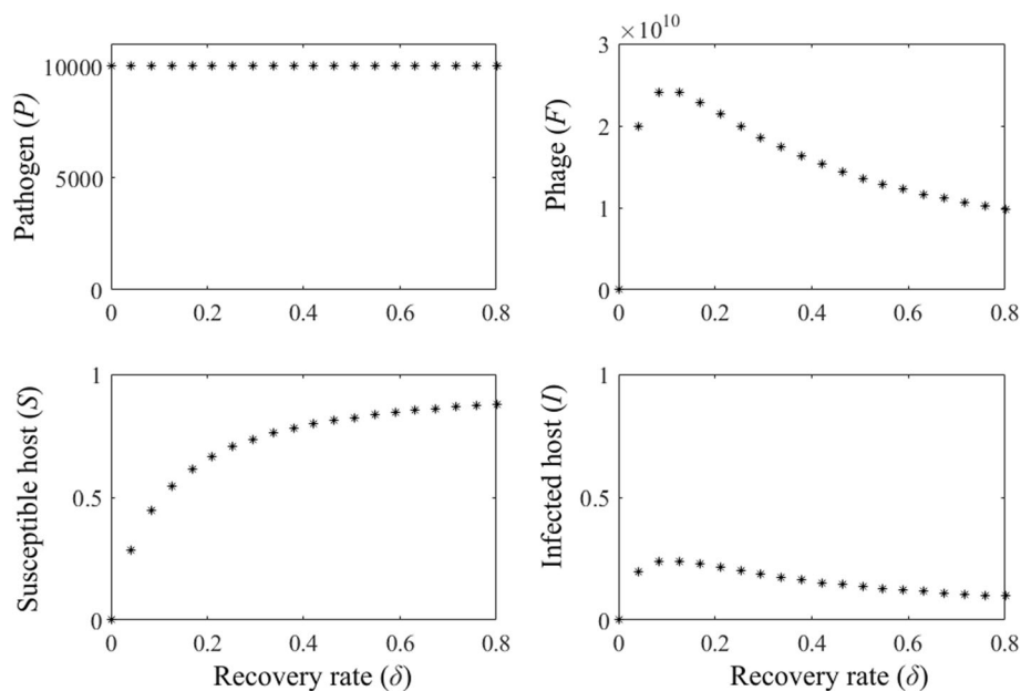
Fig. 2 Bifurcation diagrams of the model dynamics in the absence of the phage-resistant bacteria population ( B = 0 ), presenting population densities of the susceptible host ( S ), the infected hosts ( I ), the pathogen ( P ) and the bacteriophage ( F ) for the host recovery rate, 0 < \delta < 0.8 . When the recovery of hosts is not possible, the hosts are extinct. Increasing the recovery of hosts, increases the host and phage population sizes as well as the number of infections, while recovery rates above 0.2 decrease the number of infections and the population size of the phage. Pathogen populations remain stable regardless of the recovery rate of the hosts. The parameter values used are shown in Table 1
