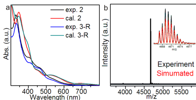
Figure 3. a) Experimental and computed UV-vis spectra of 2 and 3-R in \text{CH}_2\text{Cl}_2 . In the theoretical spectra, the individual optical transitions have been folded into a smooth curve by using a Gaussian width of 0.1 eV. b) ESI-MS of single-crystals of 3-R in \text{CH}_2\text{Cl}_2 .
