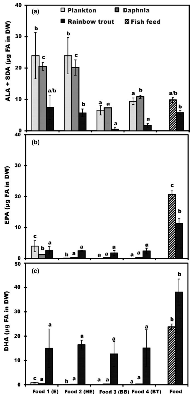
FIGURE 4 Percent abundance by mass (μg FA in mg DW \pm SD) of (A) Alpha-linolenic acid (ALA; 18:3ω3) and stearidonic acid (SDA; 18:4ω3), (B) eicosapentaenoic (EPA; 20:5ω3), and (C) docosahexaenoic (DHA; 22:6ω3) across three trophic levels (plankton, Daphnia /feed, and trouts). Number of analyzed sample ( n ) is four for all groups. Different letters (a–c) denote significant differences ( p < .05 ) among diets
