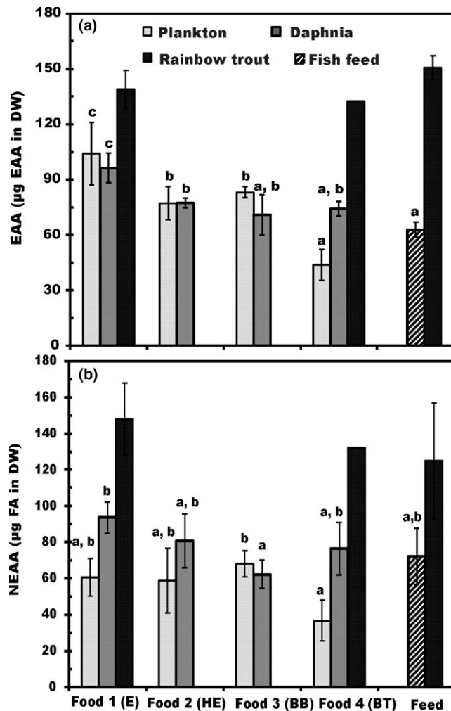
FIGURE 3 Percent abundance by mass (μg amino acids per mg DW \pm 1 SD, see text for amino acid groups) of (A) essential amino acids (EAA) and (B) nonessential amino acids (NEAA) in three trophic levels (plankton, Daphnia , and juvenile trout). Number of analyzed samples ( n ) is four for basal foods, Daphnia , and fish fed fish feed. There were only two surviving replicates of fish under treatment HE (food 2) and only one for under treatment BT (food 4). There was insufficient sample for analysis of fish treatments HE and BB (foods 2 and 3). Different letters (a–c) denote significant differences ( p < .05 ) between diets in amino acid content
