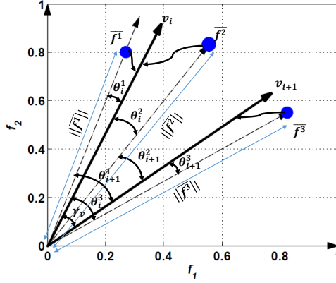
Figure 2: An illustration for assignment of individuals to a reference vector assignment and calculation of the selection criteria.
