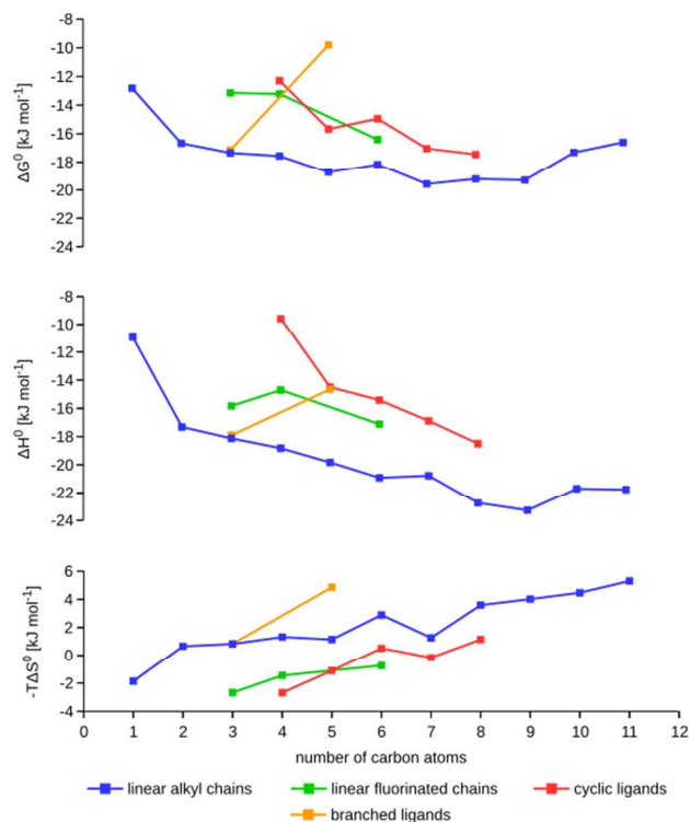
Figure 4. Gibbs free energy ( \Delta G^\circ , enthalpy ( \Delta H^\circ ), as well as entropy ( -\Delta S^\circ ) changes for the dimerization of substituted complexes [\text{Li}_3\text{L}_6\text{Ti}_2]^- in \text{DMSO-d}_6 .
