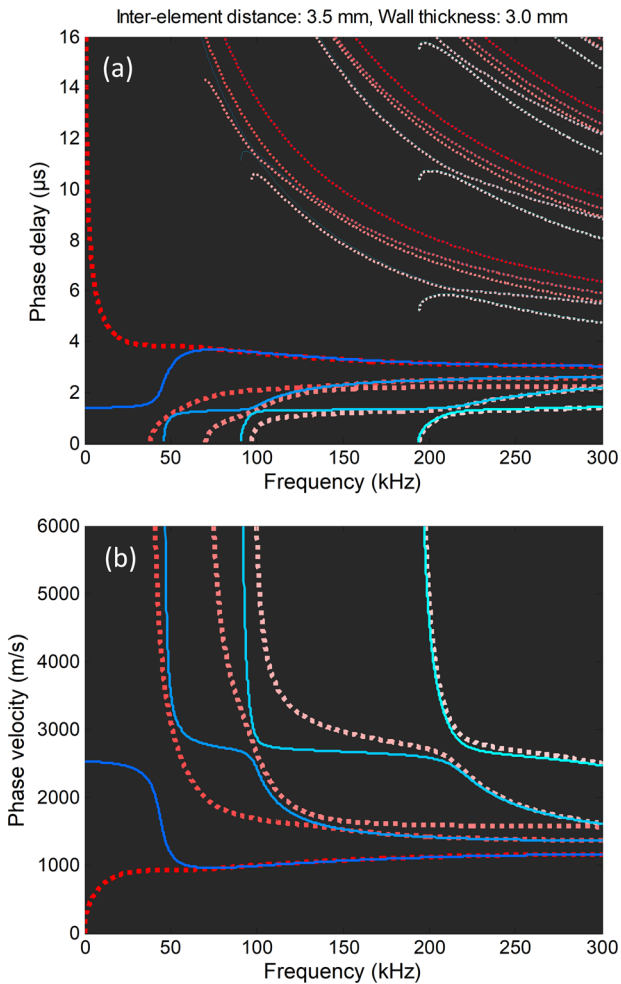
FIG. 2. Theoretically predicted (a) phase delay and (b) phase velocity as a function of frequency in a 3 mm tube with 5 mm coating. Thick lines represent results with n = 0 and thin lines results with n < 0 . Blue color tones (solid lines) represent longitudinal modes L_{LC}(0,i) and red color tones (dashed lines) fundamental flexural modes F_{LC}(1,i) . The values of index i = 1, 2, 3, 4 are indicated by descending levels of color saturation.
