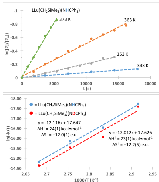
Fig 1. Top: First order plots of the thermal decomposition of complex 2 at various temperatures; Bottom: Eyring plot for the thermal decomposition of complexes 2 and 2-d
