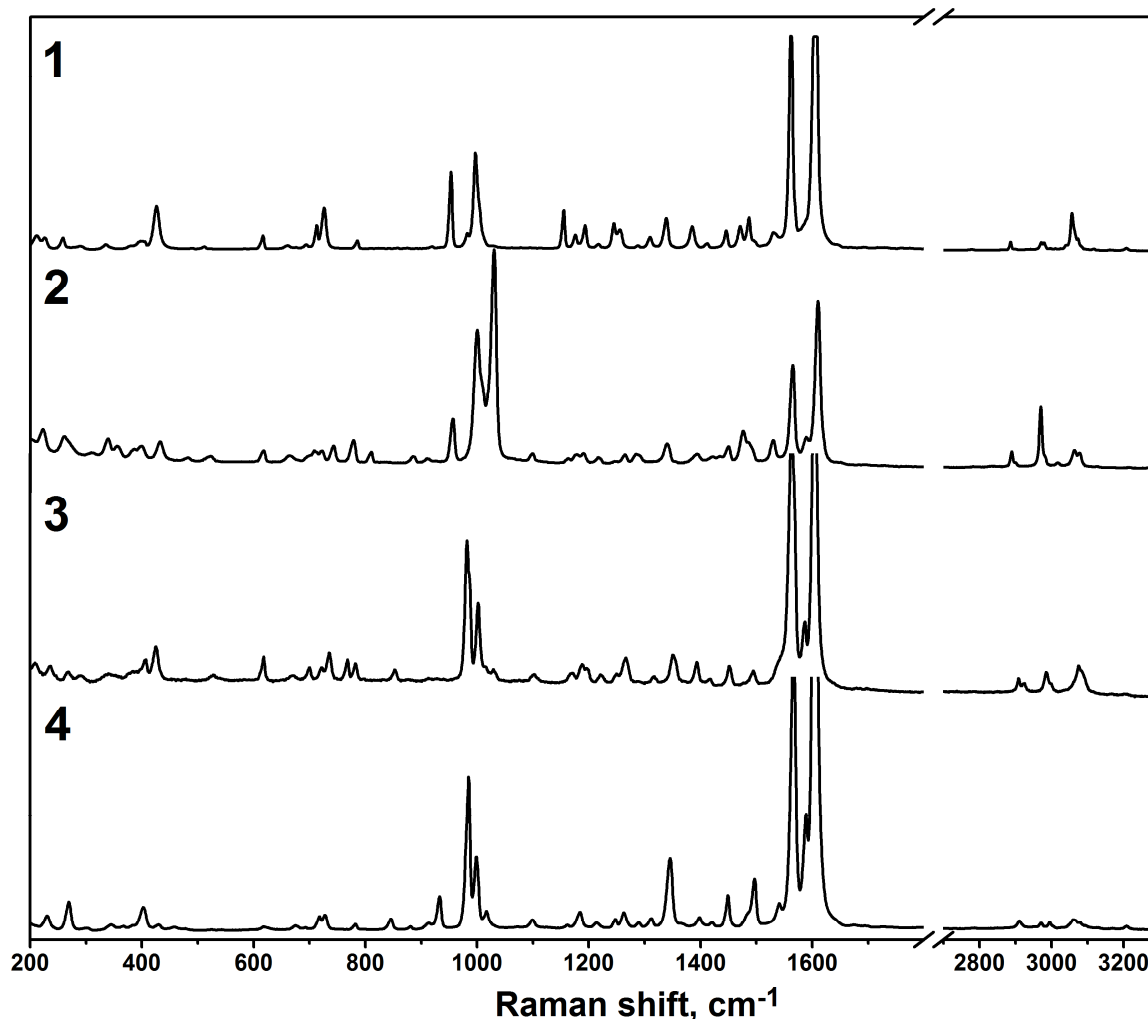
Figure 7. Raman spectra recorded on single crystals of 1 , 2 , 3 and 4 . The region 1700\text{--}2700\text{ cm}^{-1} is removed due to the absence of bands.
