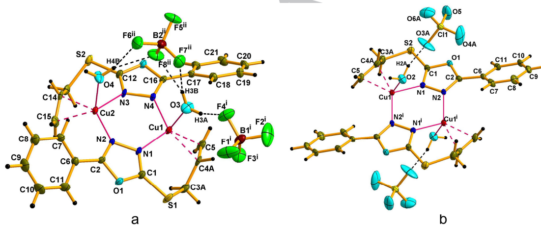
Figure 4. Part of the structure of 3 (a) and centrosymmetric fragment of 4 (b). Thermal ellipsoids are shown at 50 % probability. The disorders of the allyl group (attached to Cu2, in 3 ) and the \text{ClO}_4^- anion (in 4 ) are omitted for clarity. Selected bond length (in Å) and angle (in deg) values: 3 : Cu1–N1 2.030(2), Cu1–N4 1.994(2), Cu1–O3 2.191(2), Cu2–N2 2.002(2), Cu2–N3 2.036(2), Cu2–O4 2.191(2), Cu1– m 1 1.964(3), Cu2– m 2 1.962(2) ( m 1 and m 2 – middle point of the C4A=C5 and C14=C15 bonds), C4A–C5 1.359(4), C14–C15 1.354(3), N1–Cu1–O3 100.31(8), N4–Cu1–O3 96.11(8), N1–Cu1– m 1 113.4(1), m 1–Cu1–O3 100.1(1), m 1–Cu1–N4 129.5(1), N2–Cu2–N3 109.76(7), N2–Cu2–O4 101.33(8), N2–Cu2– m 2 127.0(1), m 2–Cu2–O4 107.0(1), m 2–Cu2–N3 113.2(1). Symmetry codes in 3 : (i) -x, 2-y, 1-z ; (ii) x, 1+y, z ; 4 : Cu1–N1 2.004(2), Cu1–N2 i 1.992(2), Cu1–O2 2.310(2), Cu1– m 1.941(2) ( m – middle point of the C4=C5 bond), C4A–C5 1.347(4), N1–N2 1.413(3), C2–C6 1.463(3), C1–N1 1.300(3), C2–N2
