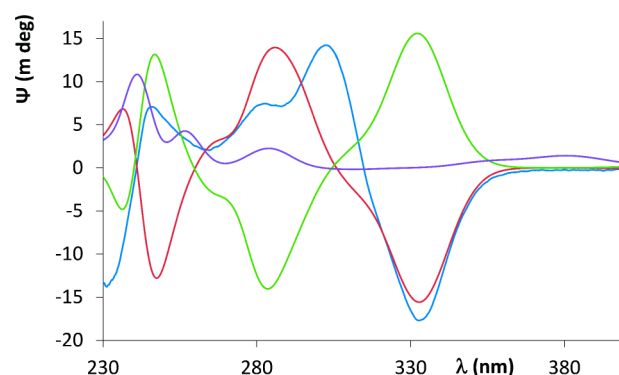
Figure 1. ECD spectra: Experimental 2 (blue), calculated for cis -fused (6aR,12aR)- 2 (red), calculated for cis -fused (6aS,12aS)- 2 (green), and calculated for trans -fused (6aR,12aS)- 2 (violet).
