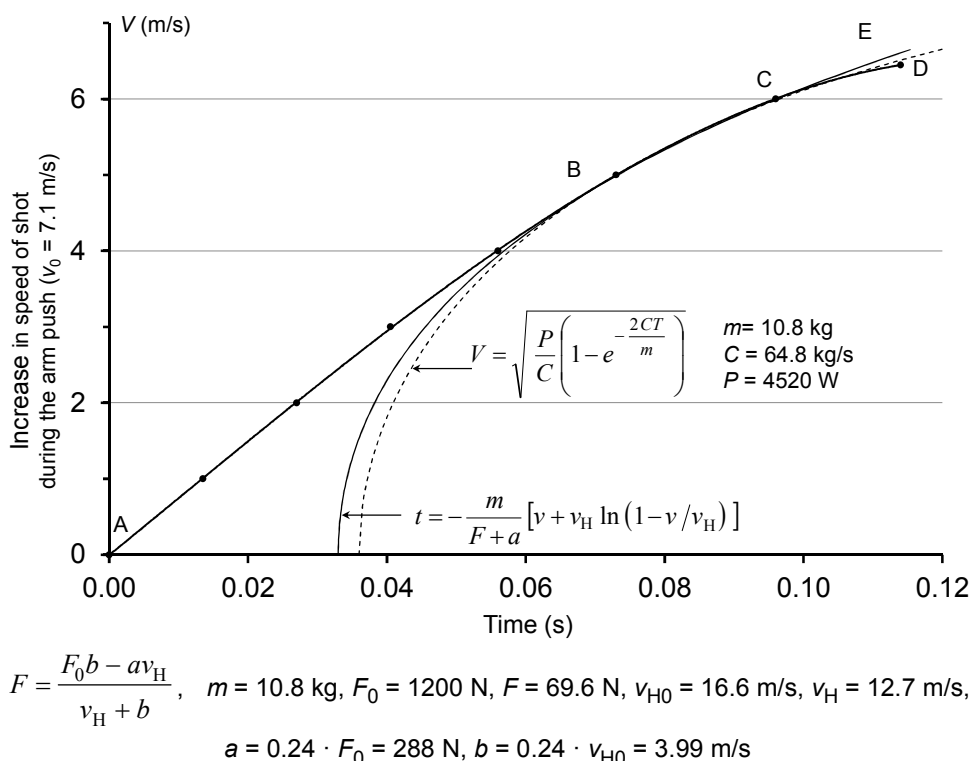
Fig. 7. The measured speed of the 20.90 m shot put (curve A – B – C – D) and the theoretical speed curves, dashed line from Eq. (21) and solid line from Eq. (11). The zero time ( T = 0 ) for theoretical curves is at 0.032 and 0.030 s, respectively
