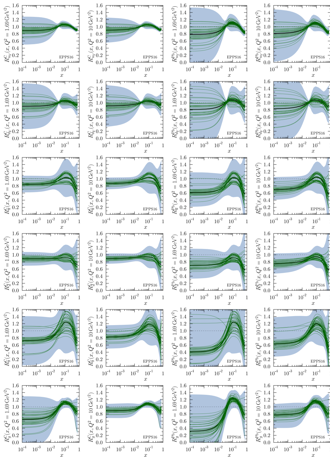
Fig. 9 The EPPS16 nuclear modifications for carbon (leftmost columns) and lead (rightmost columns) at the parametrization scale Q^2 = 1.69 \text{ GeV}^2 and at Q^2 = 10 \text{ GeV}^2 . The thick black curves corre-
