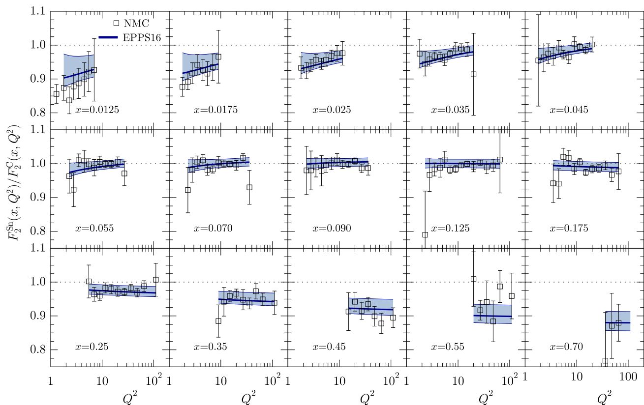
Fig. 14 The Q^2 dependence of the ratio F_2^{\text{Sn}}/F_2^{\text{C}} for various values of x as measured by NMC [79], compared with EPPS16
