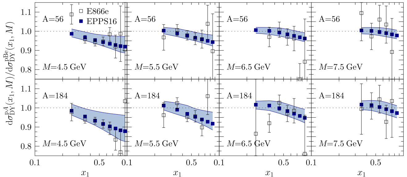
Fig. 16 Ratios of Drell-Yan dilepton cross sections d\sigma^{pA}/d\sigma^{pBe} as a function of x_1 at various values of fixed M as measured by E866 [77], compared with EPPS16
