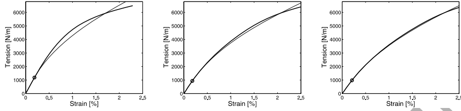
Figure 5: Examples of measured (thick line) and fitted (thin line) tension-strain curves for the RH-cycled samples. On the left is tensile test 1, in the middle is tensile test 2, and on the right is tensile test 3. The fitted yield point is marked with a circle.
