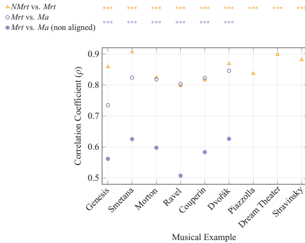
FIGURE 10. Multi-scale model correlation per stimulus comparing participant groups, segmentation tasks and alignment strategies; p values ( ***p < .001 ) obtained using Monte Carlo simulation and adjusted via Benjamini-Hochberg correction ( q = 0.05 ).
