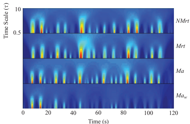
FIGURE 2. Each of the four sets of indicated boundaries was modelled via a multiple time scale approach. The kernel density over time of stimulus Morton is represented for 16 time scales.
