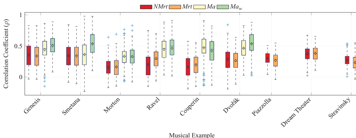
FIGURE 6. Box plot showing inter-subject correlation coefficient per stimulus for each segmentation set; p values (** p < .001 ) obtained via 10,000 Monte Carlo replications and adjusted using Benjamini-Hochberg correction ( q = 0.05 ).
