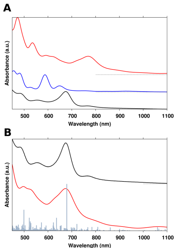
Figure 4. (A) Computed optical absorption spectra of the cluster [Ag_{67}(SPhMe_2)_{32}(PPh_3)_8]^{3+} (red) and the model cluster [Ag_{67}(SH)_{32}(PH_3)_8]^{3+} (blue) as compared to the experimental data (black). (B) The computed spectrum of [Ag_{67}(SPhMe_2)_{32}(PPh_3)_8]^{3+} blue-shifted by 95 nm (red) compared to the experiment (black). Gray sticks show the individual transitions (delta-function-like peaks showing the relative oscillator strengths). The continuous computational spectra are sums of Gaussian smoothed individual transitions (width of 0.05 eV). The intensity of the computational spectra is scaled so that the dominant peaks are approximately of similar intensity.
