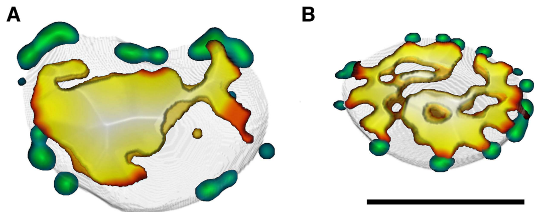
Figure 4. Spatial interaction between low-density gaps and nuclear pore complexes. Views of nuclear middle section, showing 3D reconstructions of confocal images of (A) infected and (B) non-infected cells. Images show the distribution of low-DAPI areas in comparison to Nup153-labeled NPCs (green). Low-DAPI areas denote DAPI intensity <23% of maximum. In the colour map, the low-DAPI area ranges from blue to white. Blue indicates a minimal distance whereas white indicates a maximal distance from the nuclear envelope. Scale bars, 3 \mu m.
