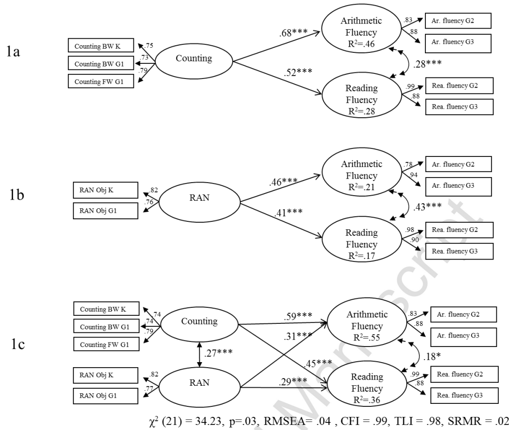
Figure 1. Standardized Estimates for models 1a-c.
