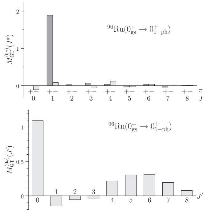
FIG. 3. The same as in Fig. 2 for the one-phonon NME M_{\text{GT}}^{(0\nu)}(0_{1\text{-ph}}^+) corresponding to the 0_1^+ state at 1148.13 keV in ^{96}\text{Mo} .
