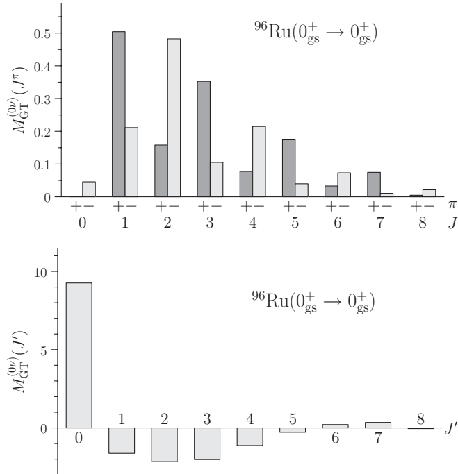
FIG. 2. Decompositions of (37) in J^\pi (upper panel) and J' (lower panel) for the ground-state Gamow-Teller M_{\text{GT}}^{(0\nu)}(0_{\text{gs}}^+) NME of ^{96}\text{Ru} . Results for the Jastrow short-range correlations are shown with g_A = 1.25 .
