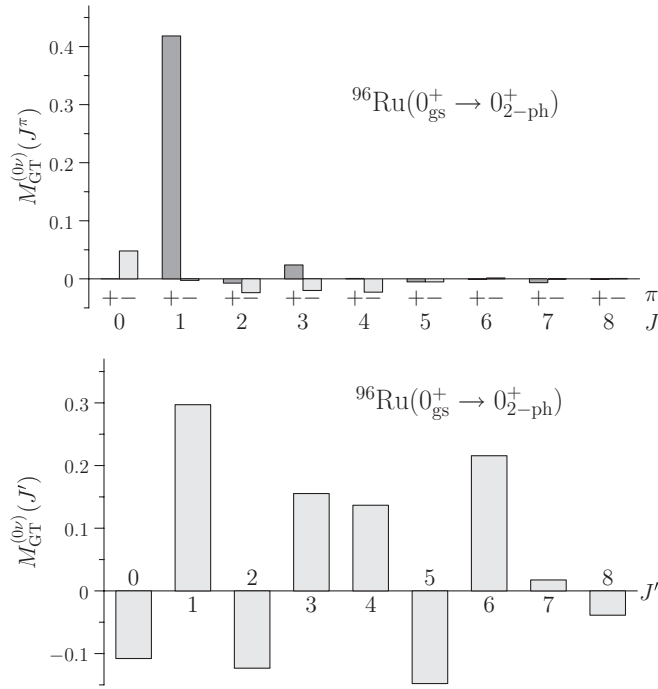
FIG. 4. The same as in Fig. 2 for the two-phonon NME M_{\text{GT}}^{(0\nu)}(0_2^+) corresponding to the 0_2^+ state at 1330 keV in ^{96}\text{Mo} .
