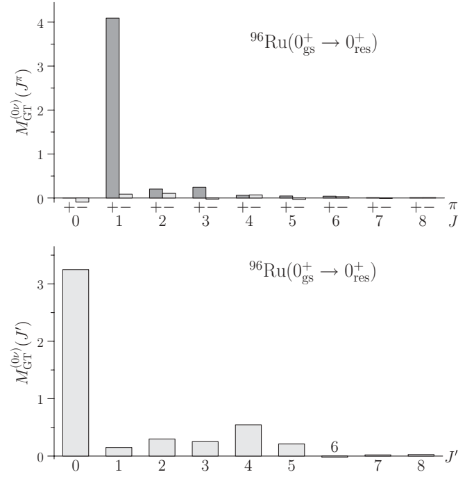
FIG. 5. The same as in Fig. 2 for the resonance NME M_{\text{GT}}^{(0\nu)}(0_{\text{res}}^+) corresponding to the 0^+ state at 2712.68 keV in ^{96}\text{Mo} .
