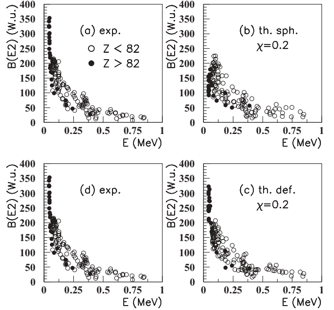
FIG. 2. Theoretical B(E2) values given by the standard spherical QRPA (b) and the dQRPA (c) versus excitation energy. For a better comparison, in panels (a) and (d) are given the same experimental B(E2) values [33].
