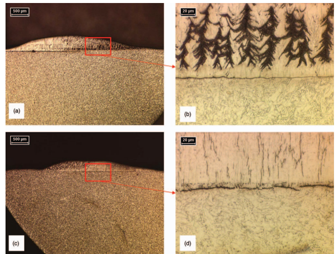
FIG. 2. (Color online) Micrograph of the Mo-cathode of the ISIS Penning source, the region facing the hydrogen injection (a) shows a dendritic growth structure (b) and the one facing Cs-injection (c) a column-like growth pattern (d). Cracks are visible between bulk and the deposited layers.
