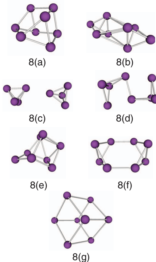
FIG. 2. Isomers of \text{Bi}_8 , (a)–(e) in order of decreasing stability. The weak “bonds” between the tetrahedra in \text{Bi}_8 (b) are 4.30 Å long.
