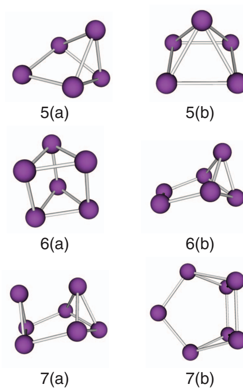
FIG. 1. Isomers of \text{Bi}_5 , \text{Bi}_6 , and \text{Bi}_7 . (a) denotes the most stable isomer, (b) the next highest in energy.
