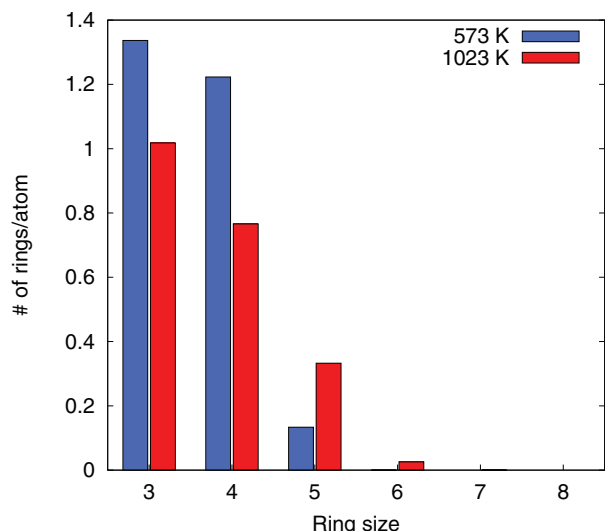
FIG. 11. Ring distributions in liquid Bi at 573 and 1023 K.
