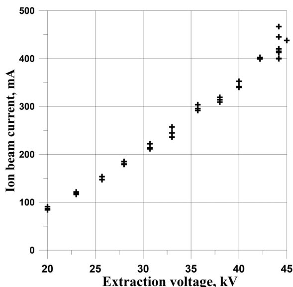
FIG. 4. Ion beam current versus extraction voltage.
