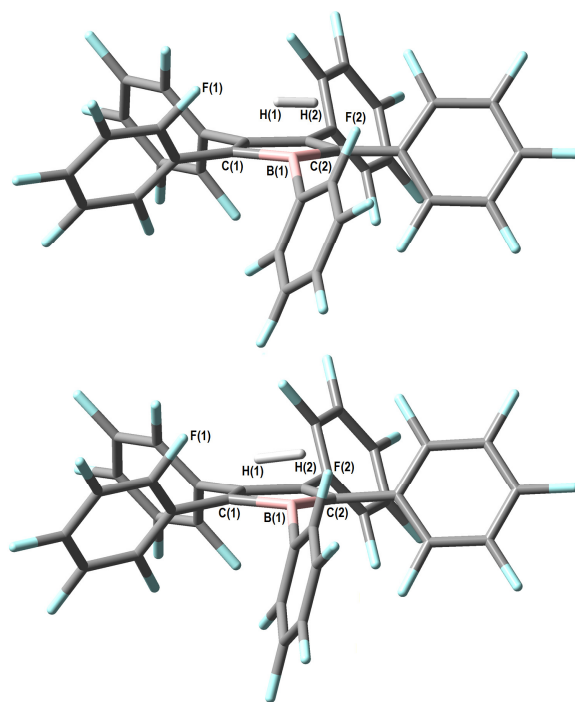
Figure 7. Computed structures for the \text{H}_2 adduct I for the fully fluorinated borole 1 (top) and the transition state TS1 (bottom) for addition of \text{H}_2 across the internal B(1)-C(1) bond to form cis-II . Selected bond lengths (Å): (top) H(1)-H(2) = 0.814; F(1)-H(1) = 2.166; F(2)-H(2) = 2.309; C(1)-H(1) = 2.056; C(2)-H(2) = 2.111; B(1)-H(1) = 1.438; B(1)-H(2) = 1.443. (bottom) H(1)-H(2) = 1.057; F(1)-H(1) = 2.266; F(2)-H(2) = 2.391; C(1)-H(1) = 1.450; C(2)-H(2) = 2.142; B(1)-H(1) = 1.328; B(1)-H(2) = 1.304.
