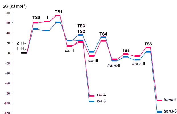
Figure 6. Calculated Gibbs free energies ( \text{kJ mol}^{-1} ) for the reaction of boroles 1 (blue) and 2 (red) with \text{H}_2 .
