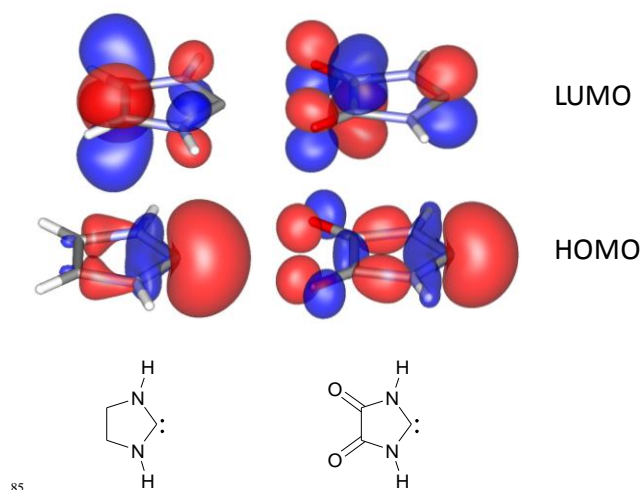
Figure 6 Frontier molecular orbitals of imidazolin-2-ylidene (left) and imidazolidin-4,5-dioxo-2-ylidene (right).
