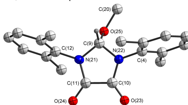
Figure 7 Molecular structure of 6b with thermal ellipsoids drawn at 50% probability. All hydrogen atoms on the 2,6-dimethylphenyl substituents have been omitted for clarity.
