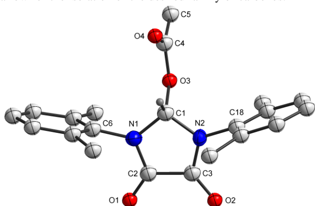
Figure 4 Molecular structure of 3c with thermal ellipsoids drawn at 50% probability. The methyl groups and the hydrogen atoms on the 2,6-diisopropylphenyl substituents have been omitted for clarity.
