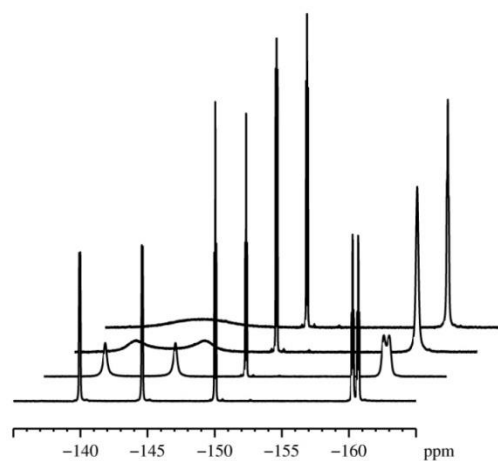
Figure 1 19 F NMR spectra of 1a at 336.0 K, 318.0 K, 288.0 K, and 248.0 K (from top to bottom, respectively).
