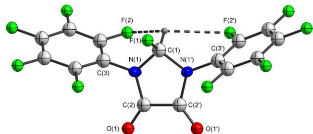
Figure 5 Molecular structure of 5a with thermal ellipsoids drawn at 50% probability.
