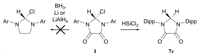
Scheme 5 Attempted reduction of 2-chloro-1,3-bis(2,6-diisopropylphenyl)imidazolidine-4,5-diones, 1 .
