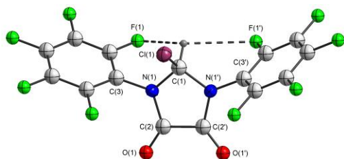
Figure 2 Molecular structure of 1a with thermal ellipsoids drawn at 50% probability.
