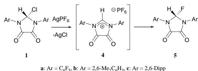
Scheme 3 Chloride abstraction from neutral 2-chloro-1,3-bis(aryl)imidazolidine-4,5-diones, 1 .
