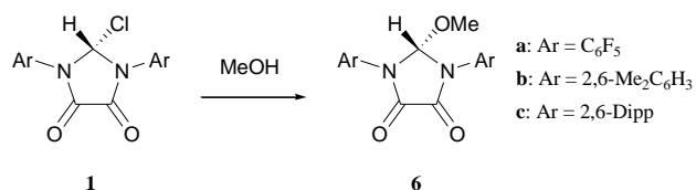
Scheme 4 Synthesis of 2-methoxy-1,3-bis(aryl)imidazolidine-4,5-diones, 6 .
