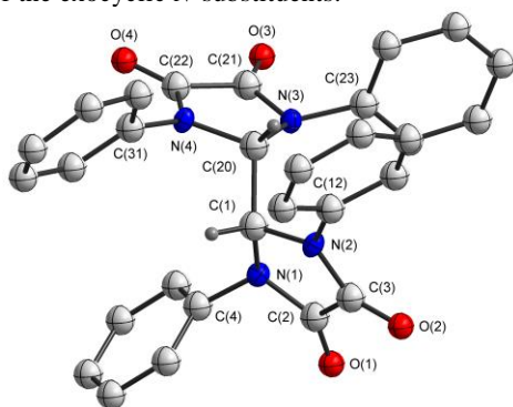
Figure 3 Molecular structure of 2b with thermal ellipsoids drawn at 50% probability. The ortho -methyl groups and the hydrogen atoms on the phenyl substituents have been omitted for clarity.
