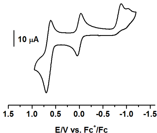
Fig. 7 Cyclic voltammogram of 1 in \text{CH}_2\text{Cl}_2 at the scan rate of 0.80\text{ Vs}^{-1} at -10\text{ }^\circ\text{C} .
