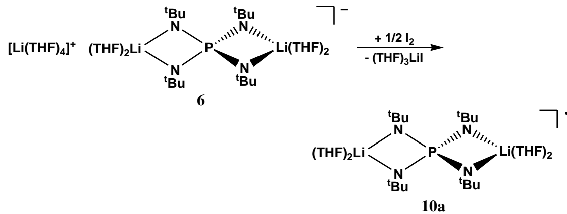
Scheme 2. Synthesis of the persistent spirocyclic radical \{(\text{THF})_2\text{Li}(\mu\text{-N}^t\text{Bu})_2\text{P}(\mu\text{-N}^t\text{Bu})\text{Li}(\text{THF})_2\}^\cdot ( 10a ).
