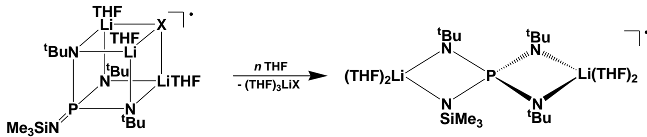
Scheme 1. Dissociation of the cubic radicals 3b and 3c to the spirocycle 8 in dilute THF solutions (X = Br, I).
