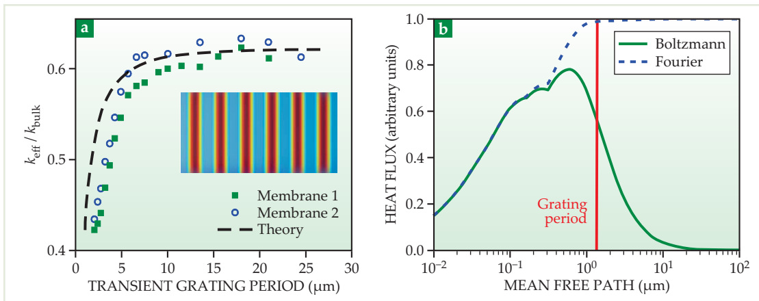
Figure 3. The thermal conductivity k_{\text{eff}} of two thin (390-nm) membranes of silicon (a), normalized to their bulk value k_{\text{bulk}} , is measured using transient grating spectroscopy, which heats the sample with the interference pattern between two laser beams. The inset illustrates the membrane's initial sinusoidal profile of alternating hot (red) and cold (blue) fringes whose temperature decay is measured in time. The thermal conductivity rapidly decreases as the grating's spatial period is reduced below 5 \mu\text{m} because some phonons have mean free paths (MFPs) comparable to that period. The scattering of phonons at membrane boundaries prohibits the measured conductivity from ever reaching the bulk value. (Adapted from ref. 10.) (b) Plotted here for a grating period of 1.5 \mu\text{m} , the spectral heat flux as a function of MFP predicted by the Boltzmann transport equation (BTE) explains the spectral reduction in thermal conductivity at low grating periods. Fourier's law breaks down for long-MFP phonons, which actually contribute far less to the thermal conductivity than the law predicts. (Adapted from ref. 11.)
