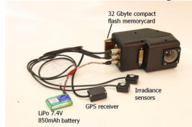
Figure 1. The Fabry-Perot interferometer spectral camera with GPS receiver, battery and irradiance sensors.
