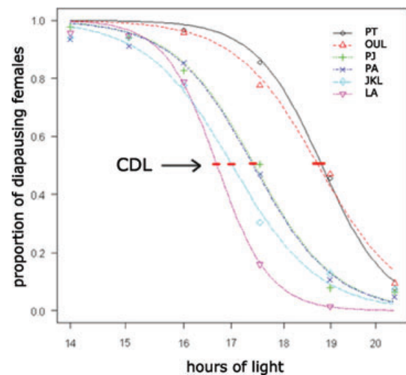
Figure 3. The graphical result of dose-response model showing correlation between latitude and average CDL for each population.
