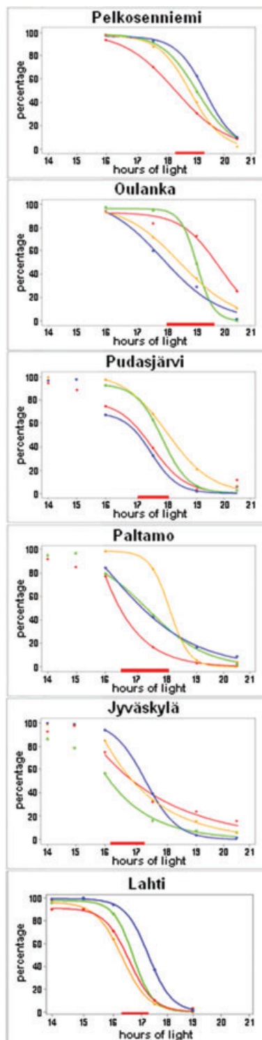
Figure 2. Proportion of diapausing females in four isofemale lines from different sampling localities in different LD cycles. Critical day length (CDL) is indicated with a thick line on the x-axes. The points not connected with the lines (on the left side of the graphs for Pudasjärvi, Paltamo, and Jyväskylä) represent the extra LD cycles used in the second set of the diapause experiment (see text for details).
